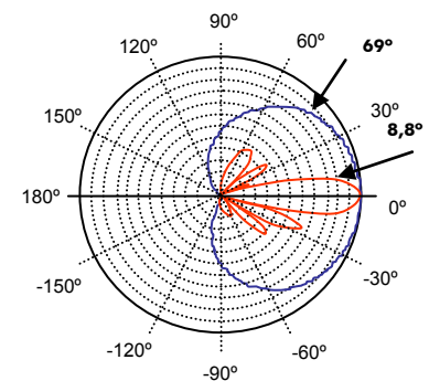
GSM900 pattern
