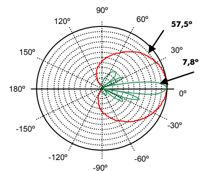
Broadband pattern
